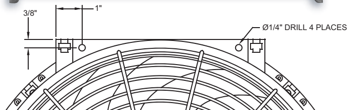
FIGURE 3 FOR USE WITH JEGS #52103 13" FANS (4) 1/4" HOLES MUST BE DRILLED IN FAN SHROUD
